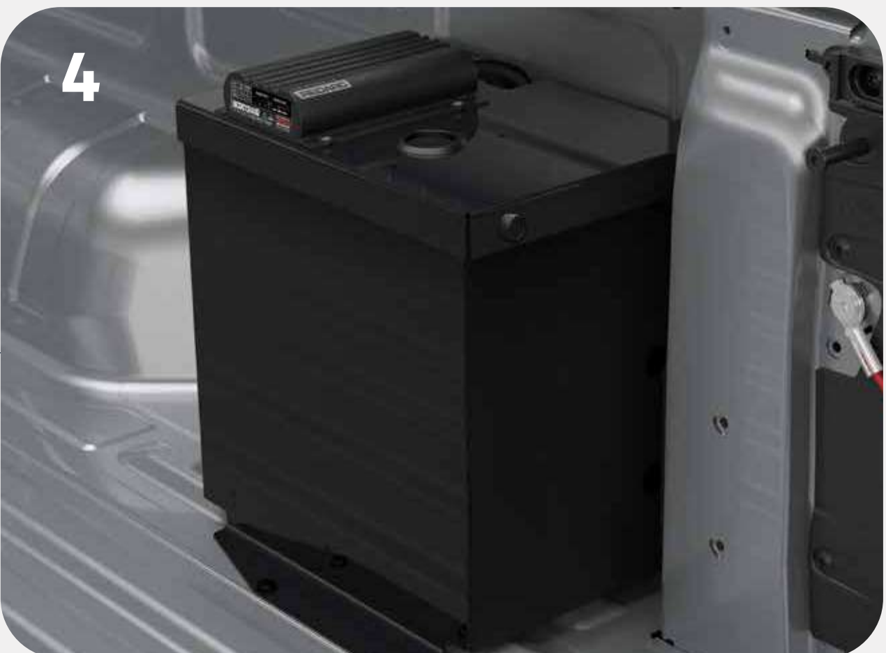
4 Auxiliary Battery Kit - Tub Mounted with 40A Charger All Variants
